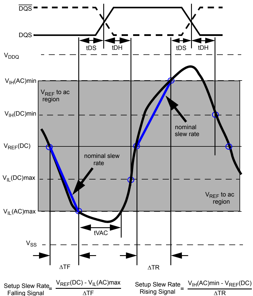
Figure 7. Illustration of nominal slew rate for tDS (differential DQS, DQS-bar)
